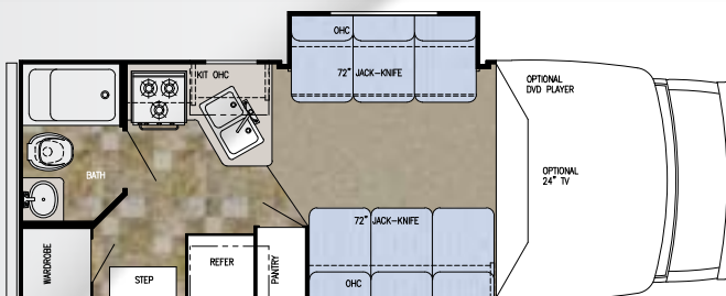
MODEL 5230
