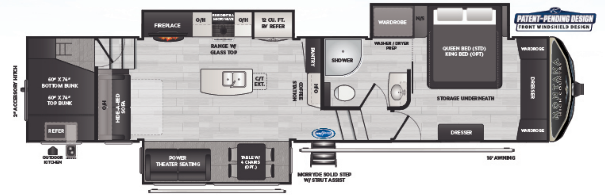
NEW! 350/351BH | Dual 60" x 74" oversized bunks and outside kitchen RV REFRIGERATOR RES. REFRIGERATOR WEIGHT:12935 LENGTH:39'
