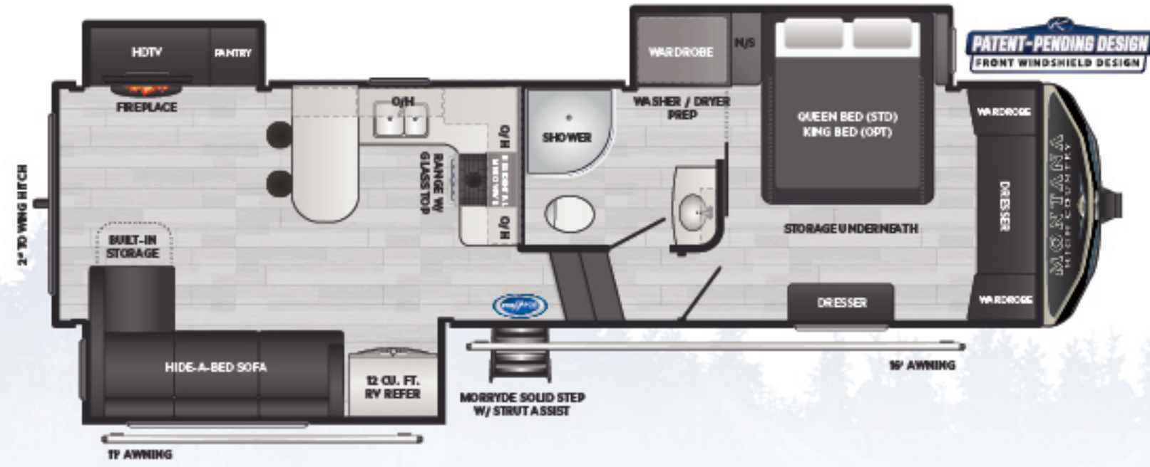
NEW! 280/281CK | Center kitchen, three slides RV REFRIGERATOR RES. REFRIGERATOR WEIGHT:10695 LENGTH:32' 2"
