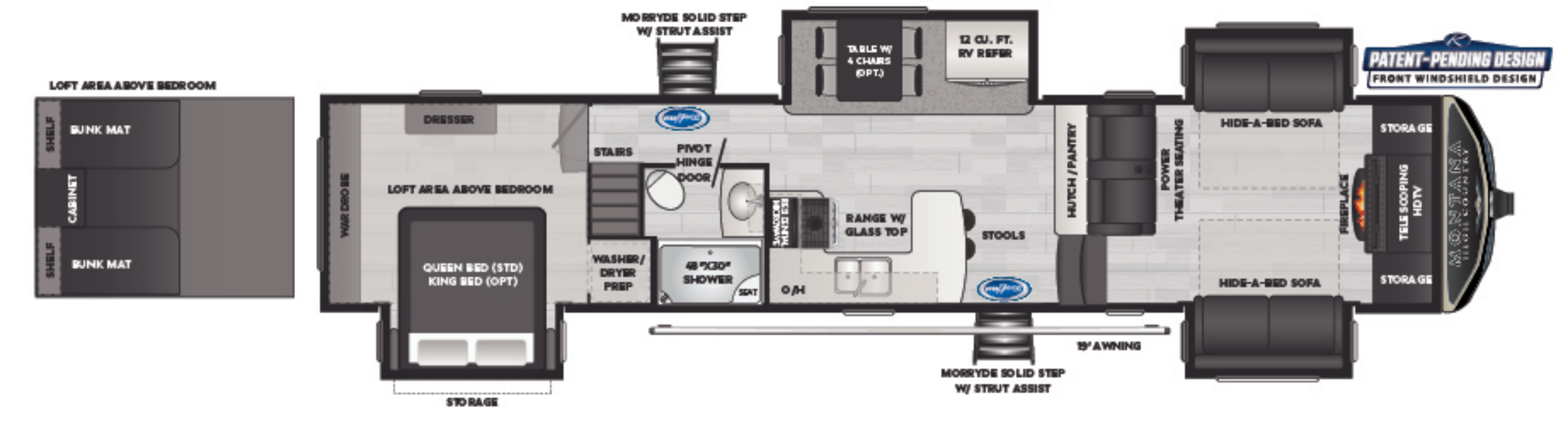
376/377FL | Front living room, four slides w/ rear overhead loft RV REFRIGERATOR RES. REFRIGERATOR WEIGHT:12985 LENGTH:41' 11"
