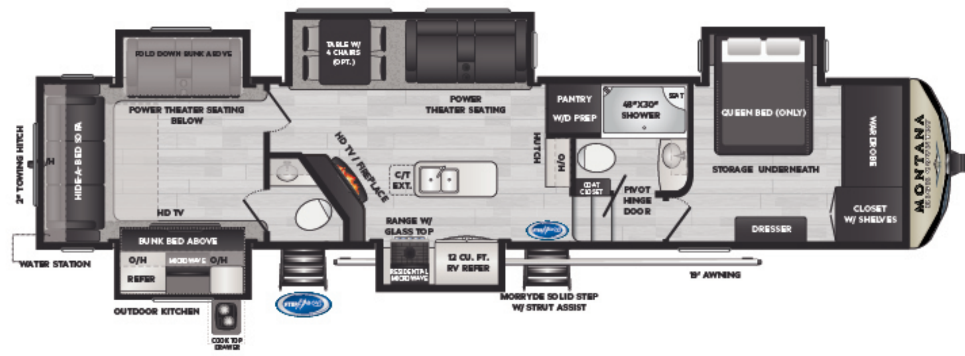
362RD | Rear den or rear bunkhouse RV REFRIGERATOR WEIGHT:13260 LENGTH:40' 1"
