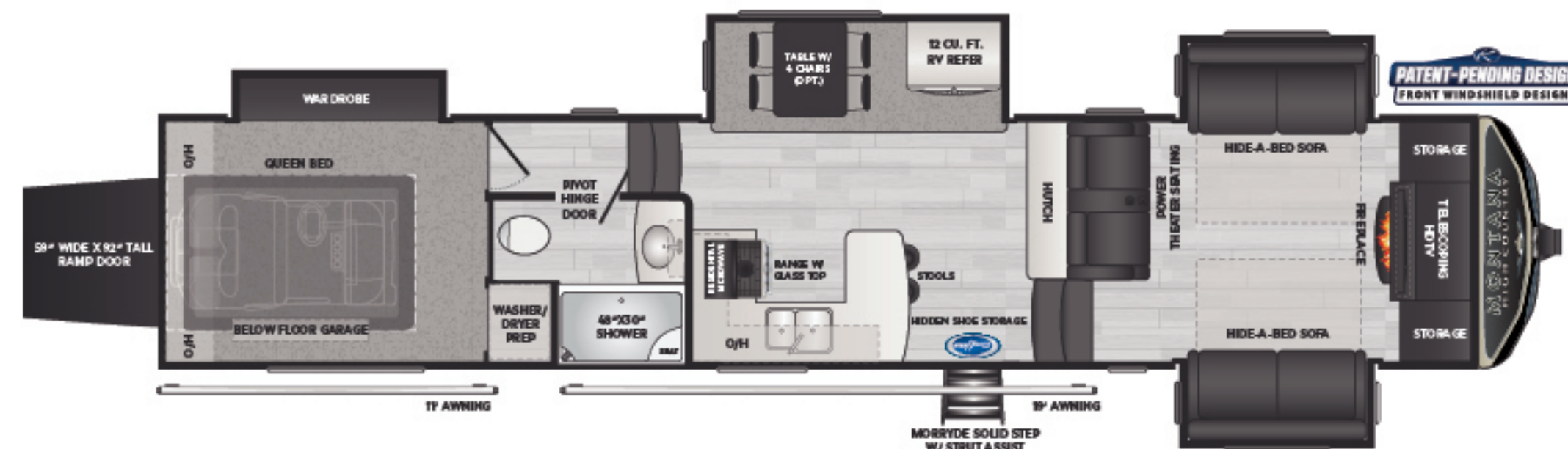
382/383TH | Front living room w/ rear garage and ramp door RV REFRIGERATOR RES. REFRIGERATOR WEIGHT:13880 LENGTH:41' 9"
