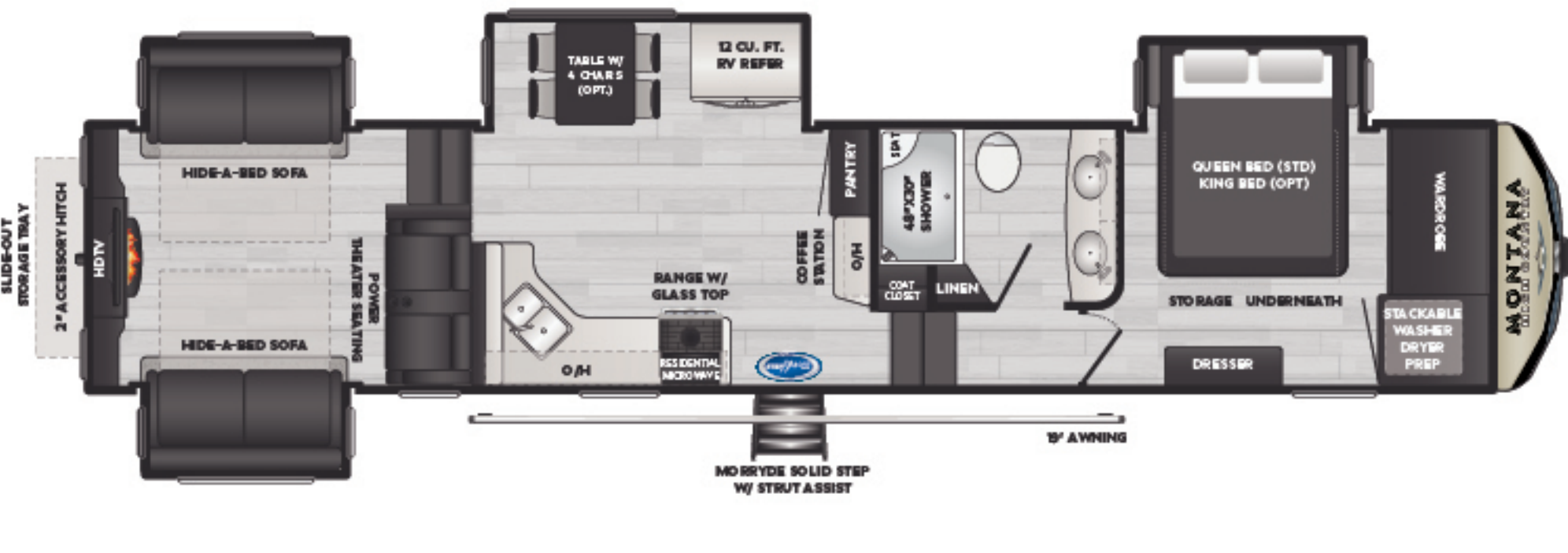
372/373RD | Elevated rear den w/ pull-out rear storage RV REFRIGERATOR RES. REFRIGERATOR WEIGHT:12939 LENGTH:41' 4"
